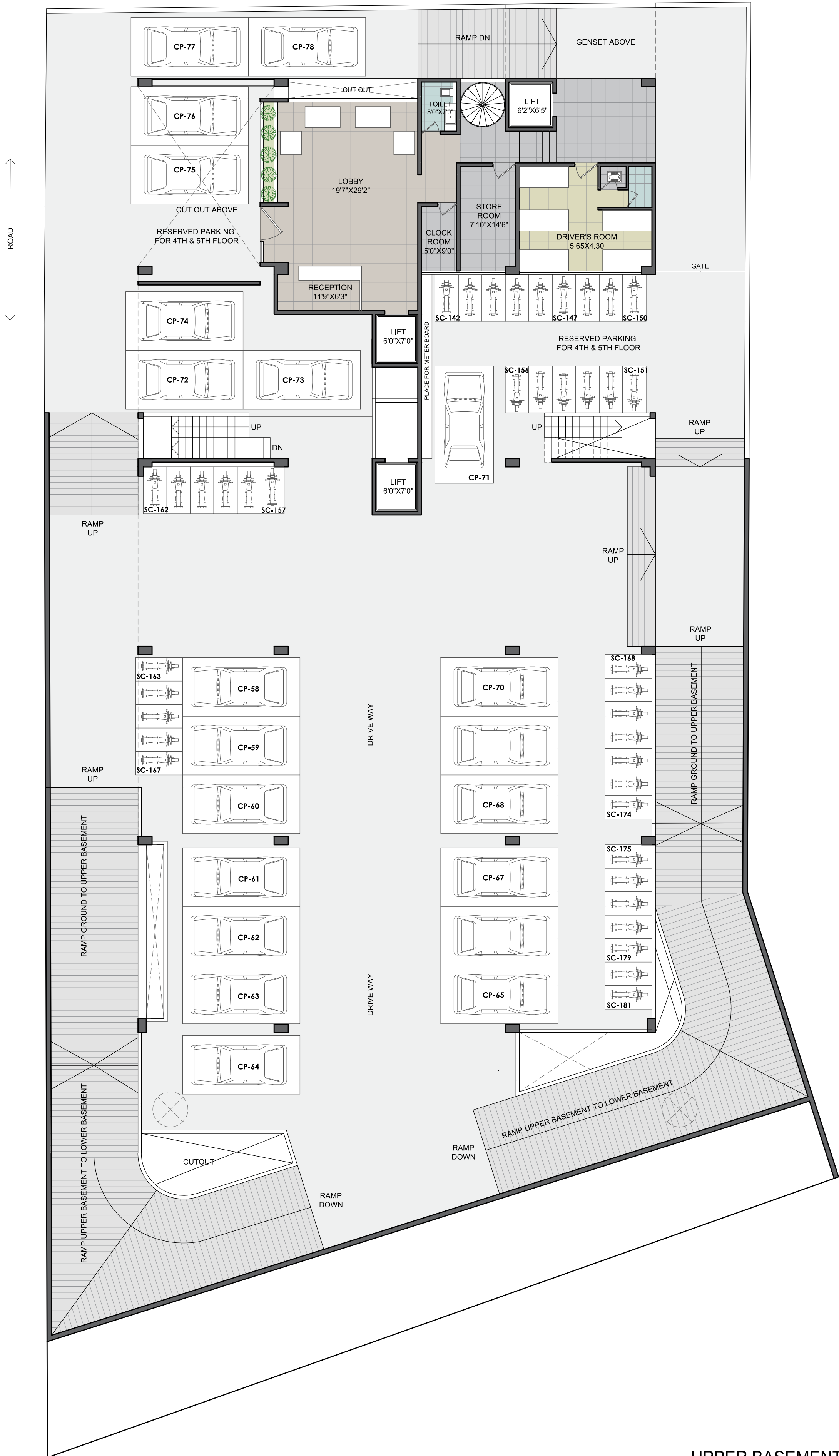
UPPER BASEMENT FLOOR PLAN
