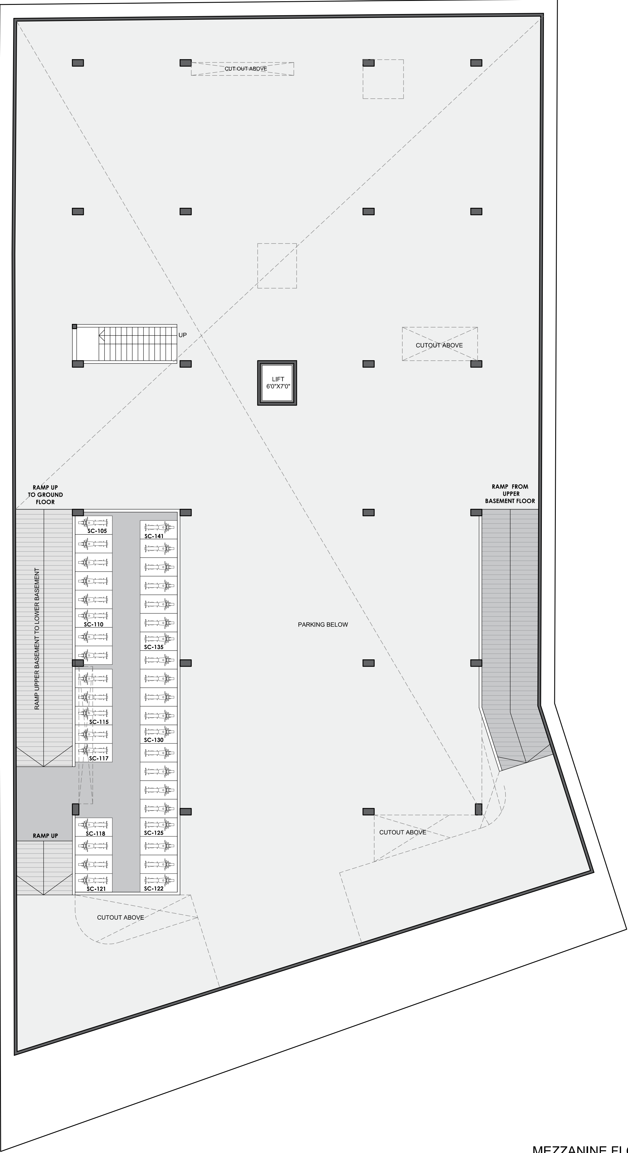
MEZZANINE FLOOR PLAN
